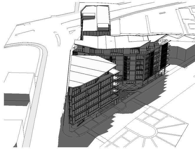
5 SUN STUDY - PROPOSED VIEW 01 - DECEMBER 21st - 4pm
