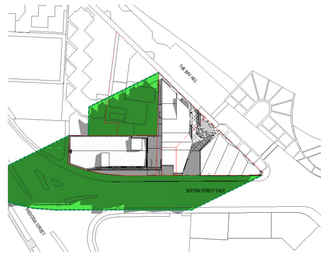
2 SUN STUDY - PROPOSED BUILDING - SEPTEMBER 21st - 9am Scale: 1:1000
