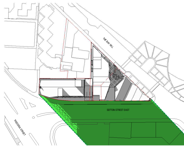
10 SUN STUDY - PROPOSED BUILDING - JUNE 21st - 4pm Scale: 1:1000
