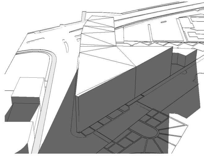
3 SUN STUDY - COMPLIANT VIEW 01 - MARCH 21st - 6pm
