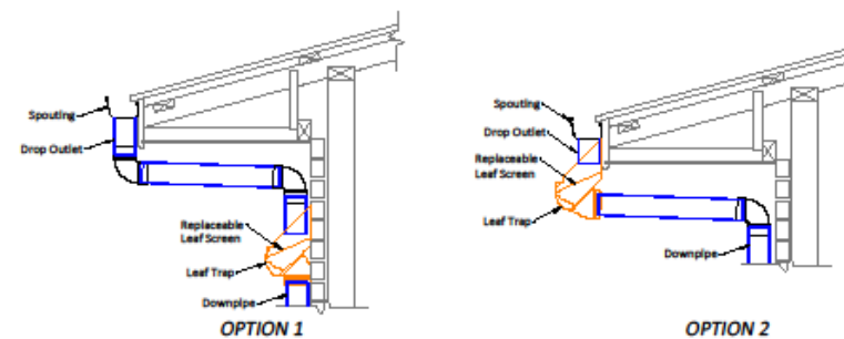
TYPICAL LEAF TRAP INSTALLATION Scale: 1:10 @ A1
