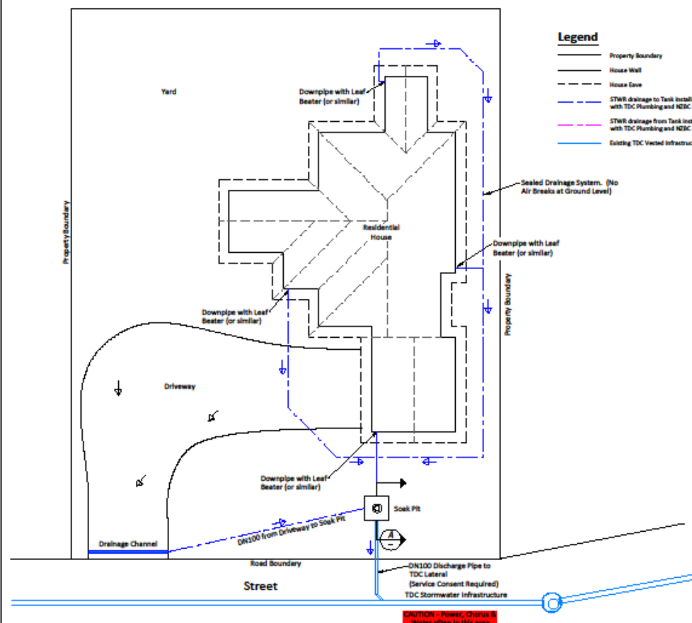
EXAMPLE DRAINAGE SITE LAYOUT Scale: 1:100 @ A1
