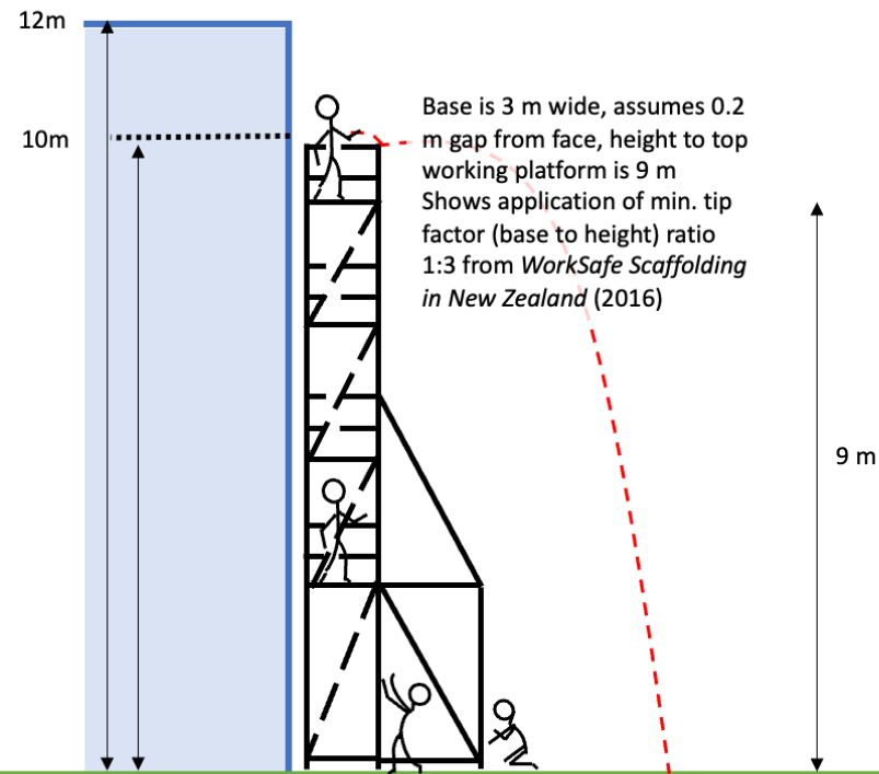
Example of a Scaffold with an explanation of the 1:3 (Base : Height) Tip Factor
