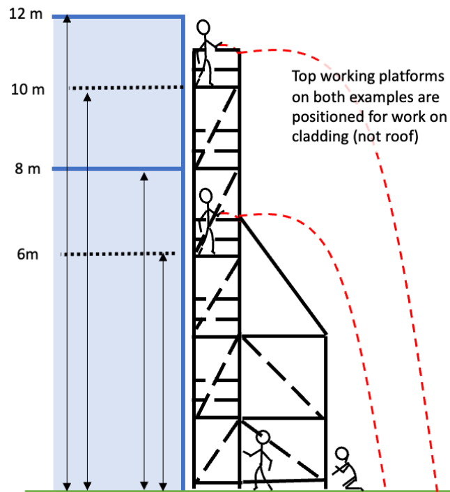
Example of a Scaffold Accessing up to 12m
