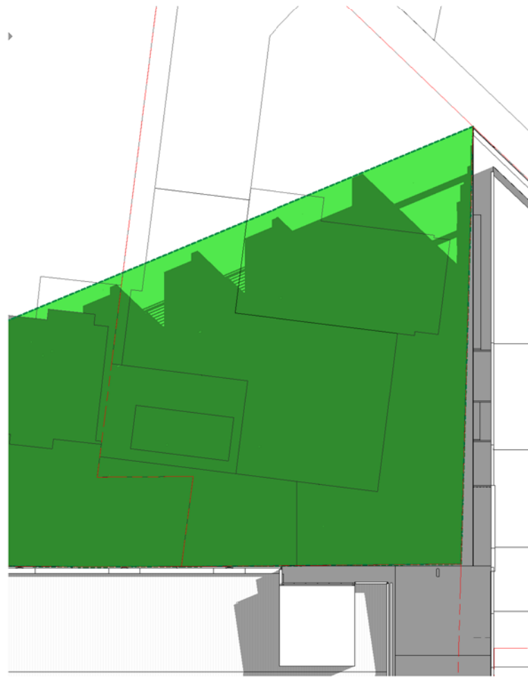
1 SUN STUDY - PROPOSED BUILDING - MARCH 21st - 9am Scale: 1:200
