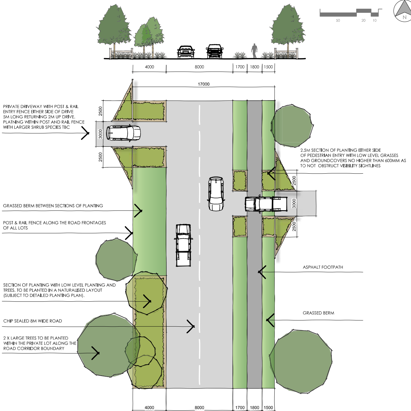
TYPICAL ROAD CORRIDOR PLAN SCALE: NTS
